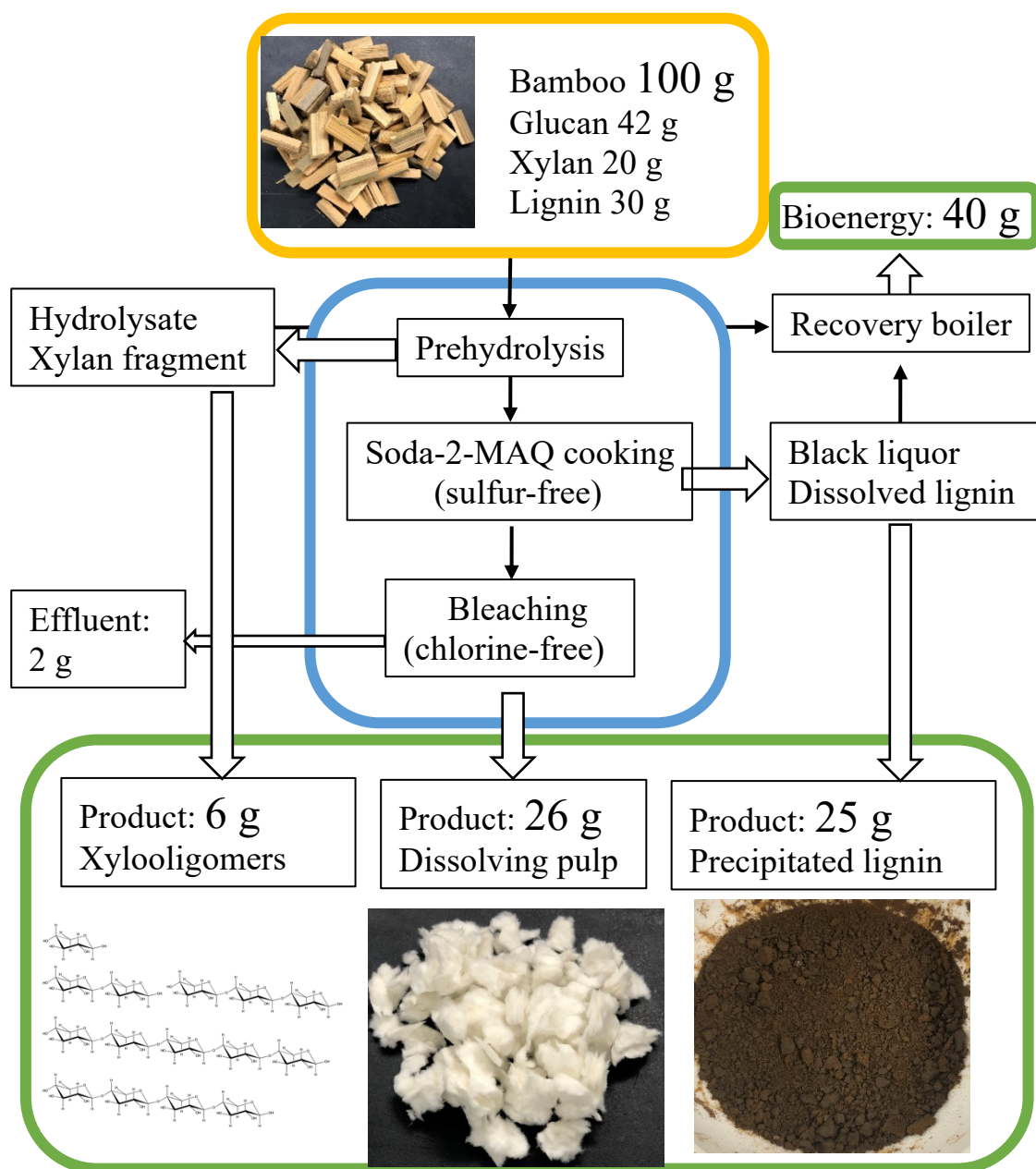
Figure 2-5 Bamboo biorefinery by prehydrolysis soda-2-methylanthraquinone (MAQ)
