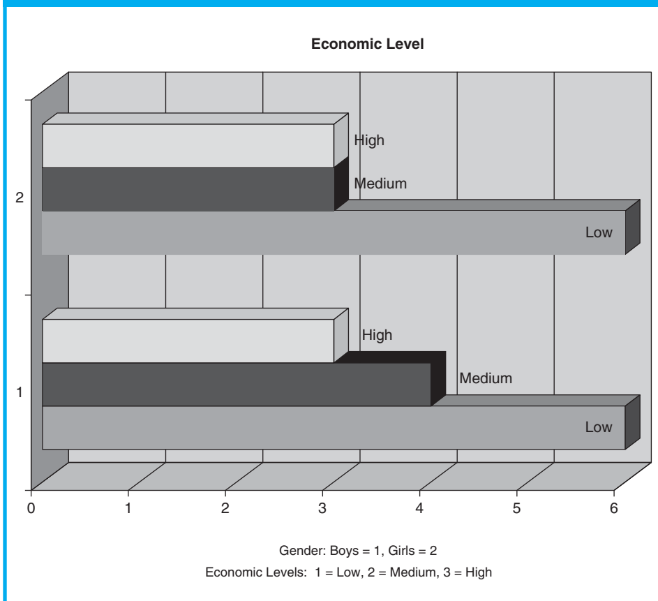
FIGURE 12.3 • Bar chart: Gender by economic level
