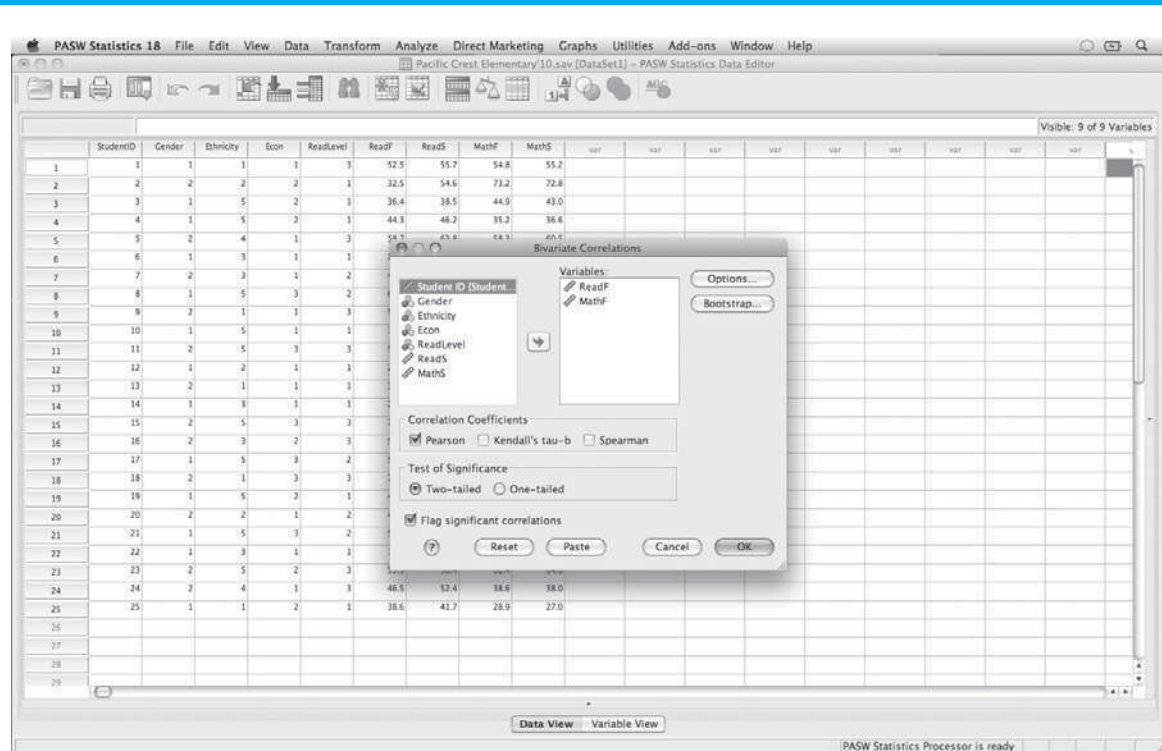
FIGURE B.12.6 • Variable selection for correlation
