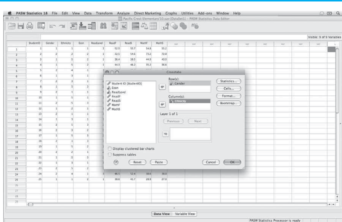
FIGURE B.12.2 • Continued
