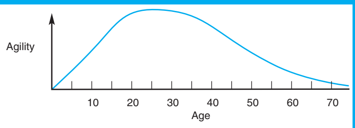
FIGURE 8.2 • The curvilinear relationship between age and agility
