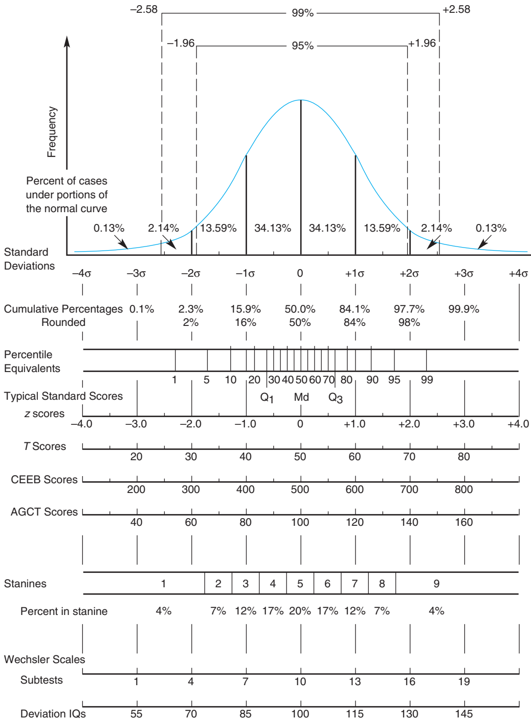
FIGURE 12.1 • Characteristics of the normal curve
