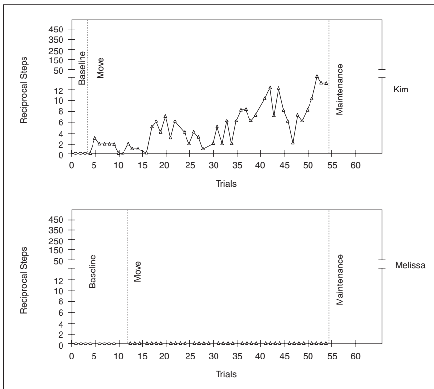
Figure 1 Independent Walking for Kim and Melissa Across Baseline, Intervention, and Maintenance Phases
