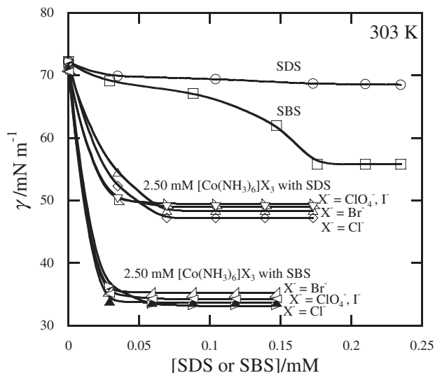
Figure 2. Surface tensions of aqueous SDS and SBS solutions with [\text{Co}(\text{NH}_3)_6]\text{X}_3 (2.50 mM) ( \text{X}^- = \text{Cl}^- , \text{Br}^- , \text{I}^- , or \text{ClO}_4^- ) at 303 \pm 0.1 K: (○) SDS, (□) SBS, (◇) SDS with [\text{Co}(\text{NH}_3)_6]\text{Cl}_3 , (△) SDS with [\text{Co}(\text{NH}_3)_6]\text{Br}_3 , (▵) SDS with [\text{Co}(\text{NH}_3)_6]\text{I}_3 , (▽) SDS with [\text{Co}(\text{NH}_3)_6](\text{ClO}_4)_3 , (▷) SBS with [\text{Co}(\text{NH}_3)_6]\text{Cl}_3 , (◁) SBS with [\text{Co}(\text{NH}_3)_6]\text{Br}_3 , (▲) SBS with [\text{Co}(\text{NH}_3)_6]\text{I}_3 , (◄) SBS with [\text{Co}(\text{NH}_3)_6](\text{ClO}_4)_3 .
