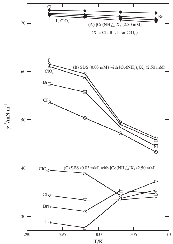
Figure 3. Surface tension values ( \gamma ) of (A) [\text{Co}(\text{NH}_3)_6]\text{X}_3 (2.50 mM) and plateaued values of surface tensions ( \gamma^* ) for (B) SDS, or (C) SBS, aqueous solutions with [\text{Co}(\text{NH}_3)_6]\text{X}_3 (2.50 mM) ( \text{X}^- = \text{Cl}^- , \text{Br}^- , \text{I}^- , or \text{ClO}_4^- ) as a function of temperature (K): (◆) [\text{Co}(\text{NH}_3)_6]\text{Cl}_3 , (▲) [\text{Co}(\text{NH}_3)_6]\text{Br}_3 , (●) [\text{Co}(\text{NH}_3)_6]\text{I}_3 , (▼) [\text{Co}(\text{NH}_3)_6](\text{ClO}_4)_3 , (○) SDS with [\text{Co}(\text{NH}_3)_6]\text{Cl}_3 , (□) SDS with [\text{Co}(\text{NH}_3)_6]\text{Br}_3 , (◇) SDS with [\text{Co}(\text{NH}_3)_6]\text{I}_3 , (△) SDS with [\text{Co}(\text{NH}_3)_6](\text{ClO}_4)_3 , (▽) SBS with [\text{Co}(\text{NH}_3)_6]\text{Cl}_3 , (▵) SBS with [\text{Co}(\text{NH}_3)_6]\text{Br}_3 , (◁) SBS with [\text{Co}(\text{NH}_3)_6]\text{I}_3 , (▷) SBS with [\text{Co}(\text{NH}_3)_6](\text{ClO}_4)_3 .
